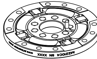
DRAWING IN THIRD ANGLE PROJECTION
